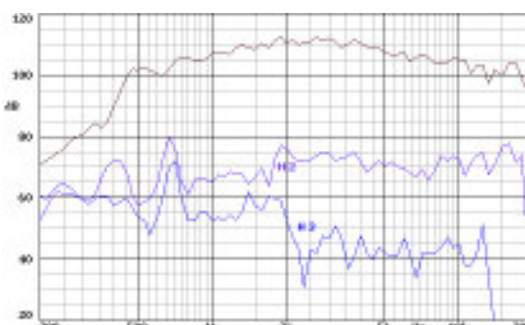
Note: on axis frequency response measured coupled to TD-565 in anechoic chamber, 1w @ 1m.
